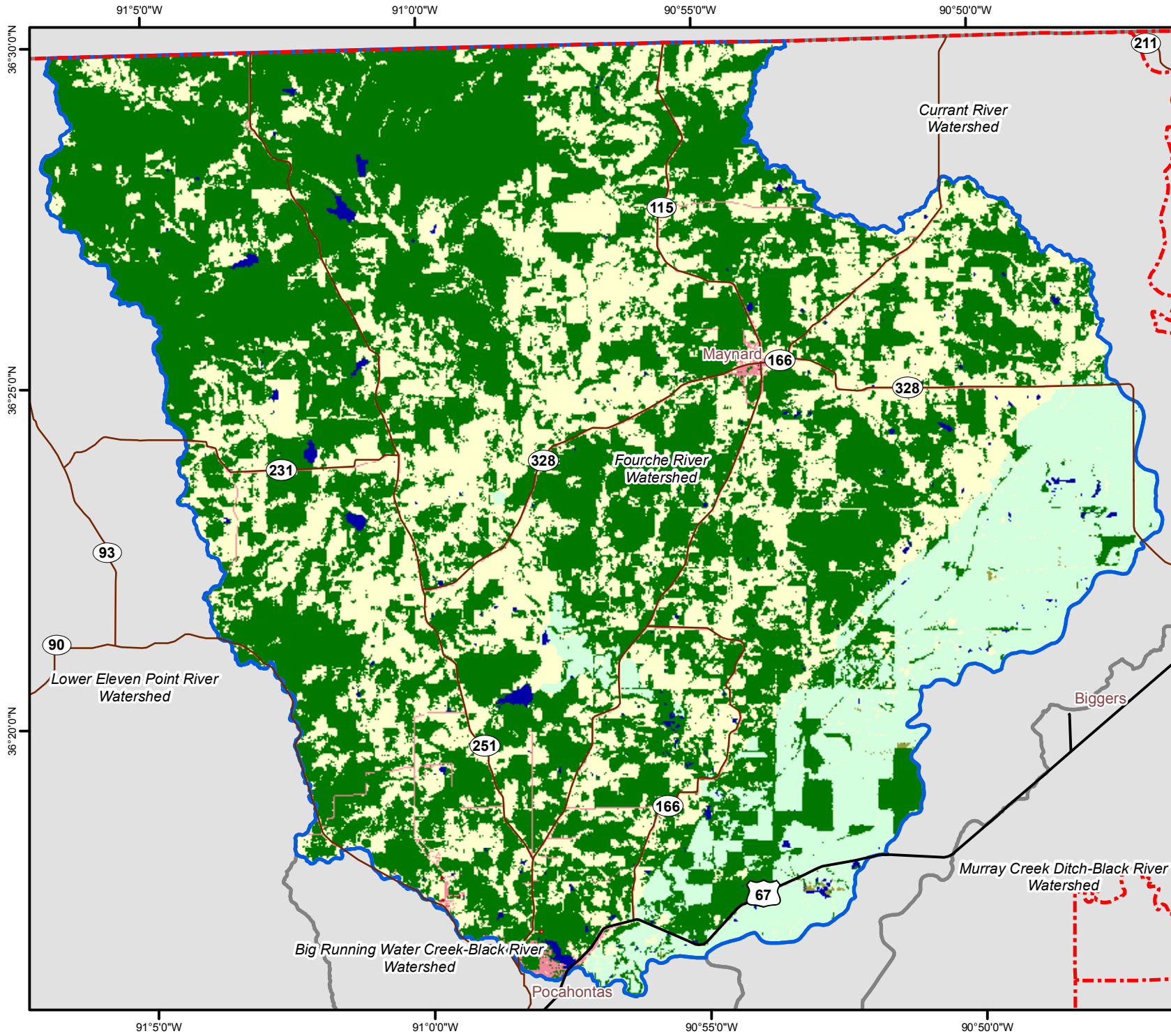
Fourche River Land Use / Land Cover, 1999
