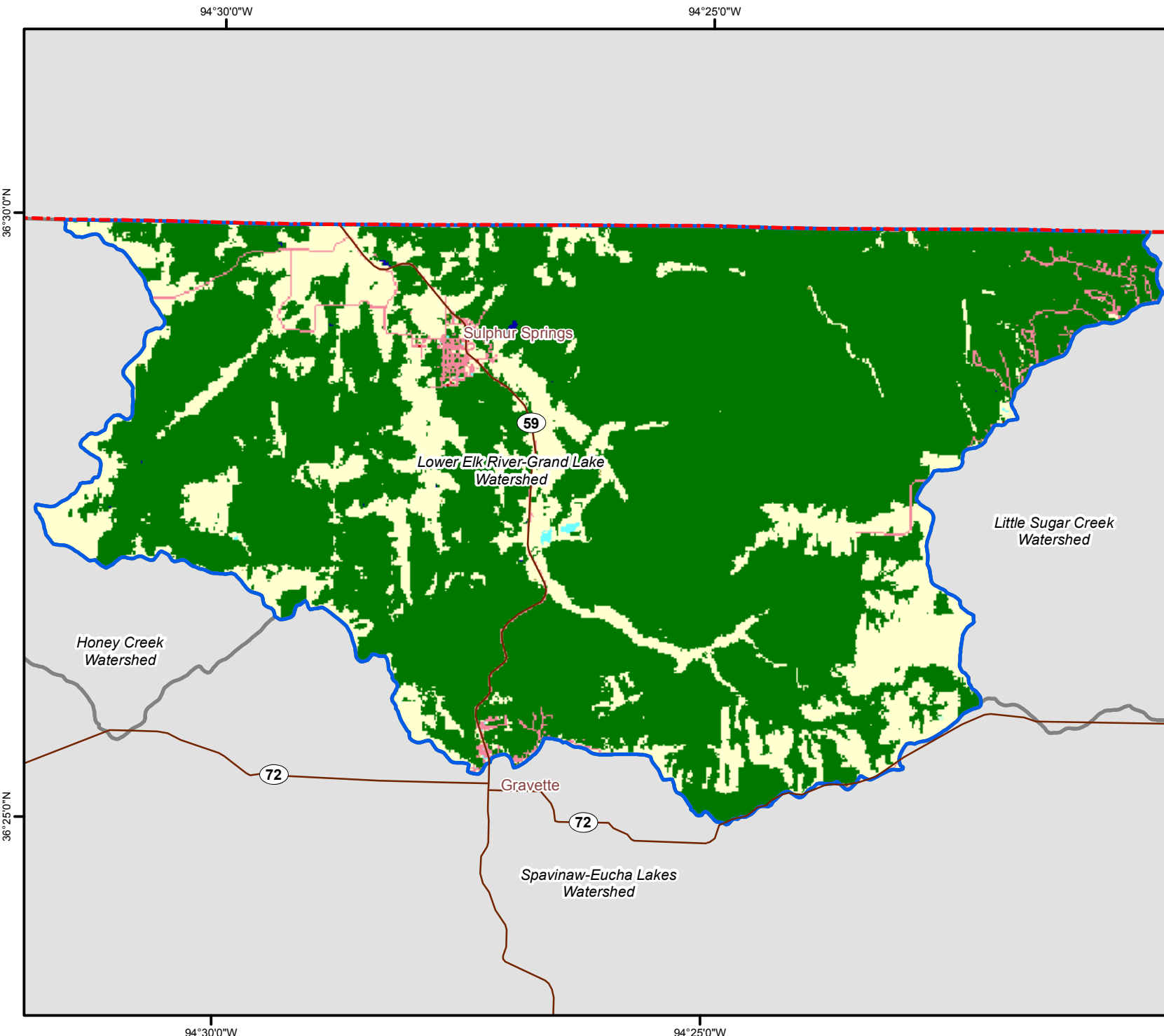
Lower Elk River-Grand Lake Land Use / Land Cover, 1999
