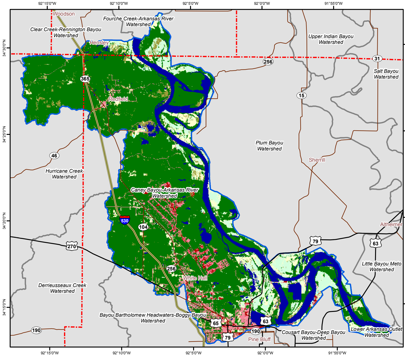
Caney Bayou-Arkansas River Land Use / Land Cover, 1999
