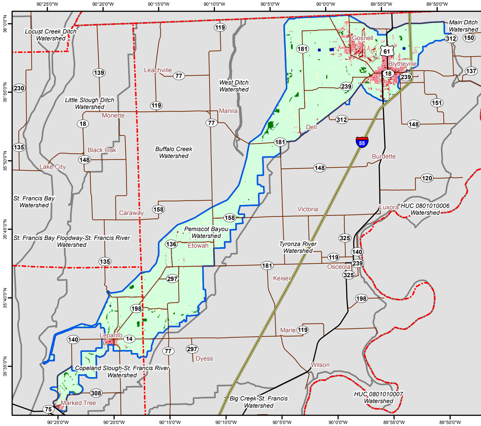
Pemiscot Bayou Land Use / Land Cover, 2004
