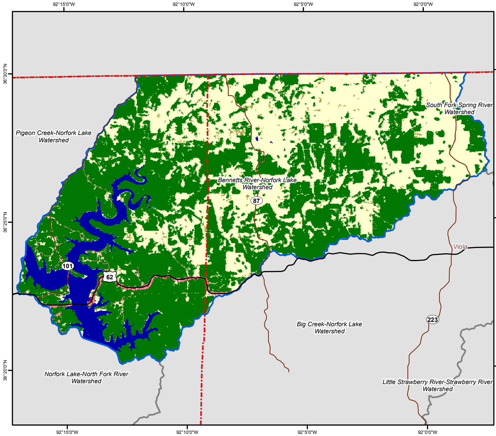
Bennetts River-Norfolk Lake Land Use / Land Cover, 2004
