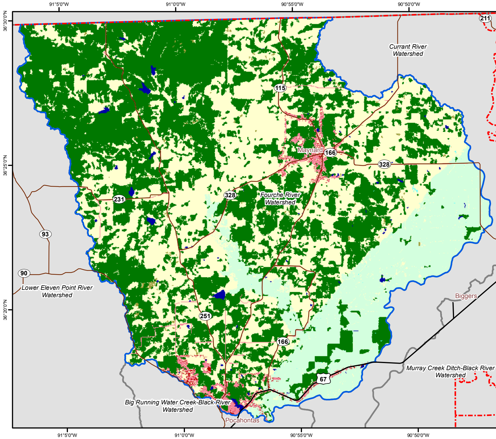
Fourche River Land Use / Land Cover, 2004
