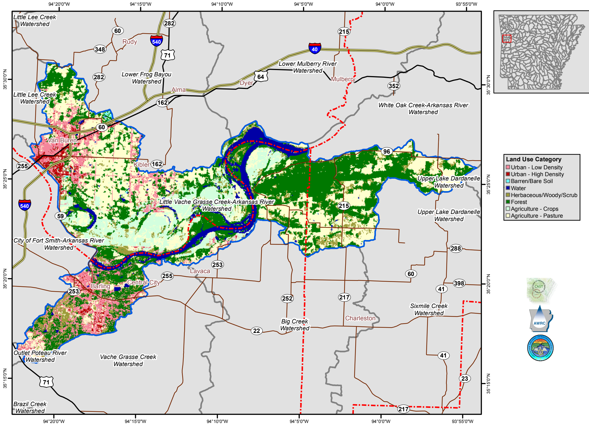
Little Vache Grasse Creek-Arkansas River Land Use / Land Cover, 2004
