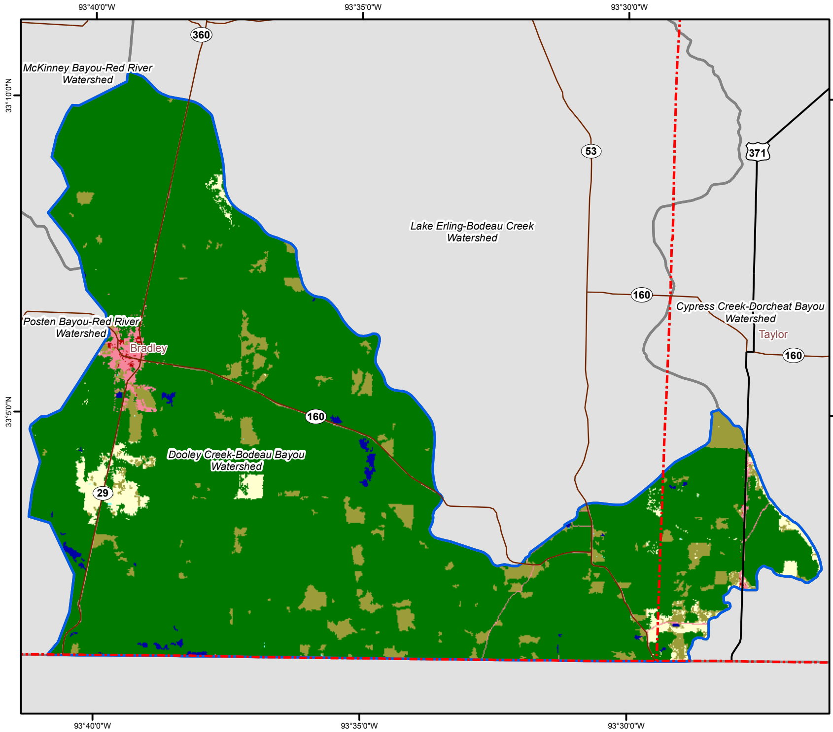
Dooley Creek-Bodeau Bayou Land Use / Land Cover, 2004
