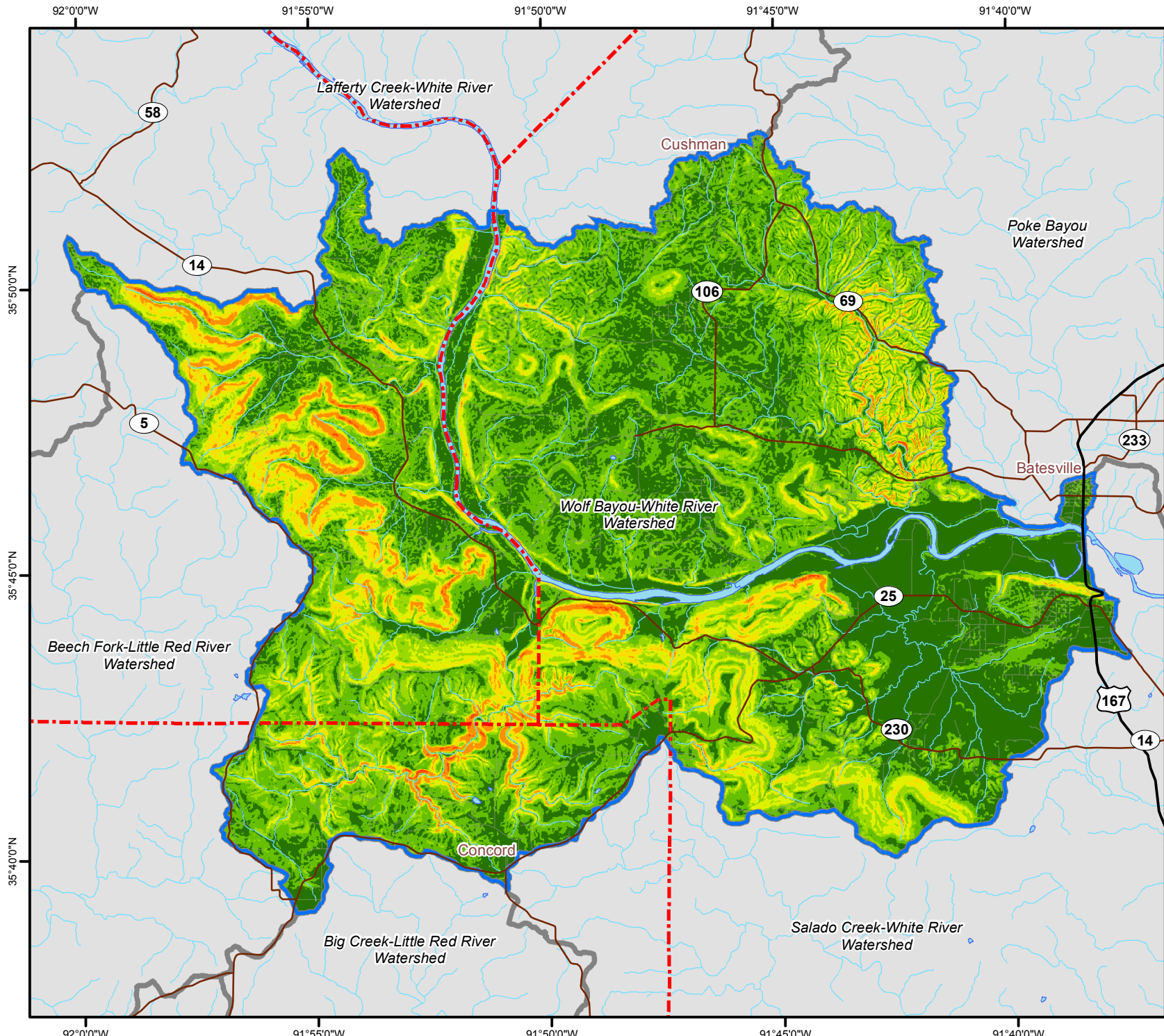
Wolf Bayou-White River Slope (Degrees)
