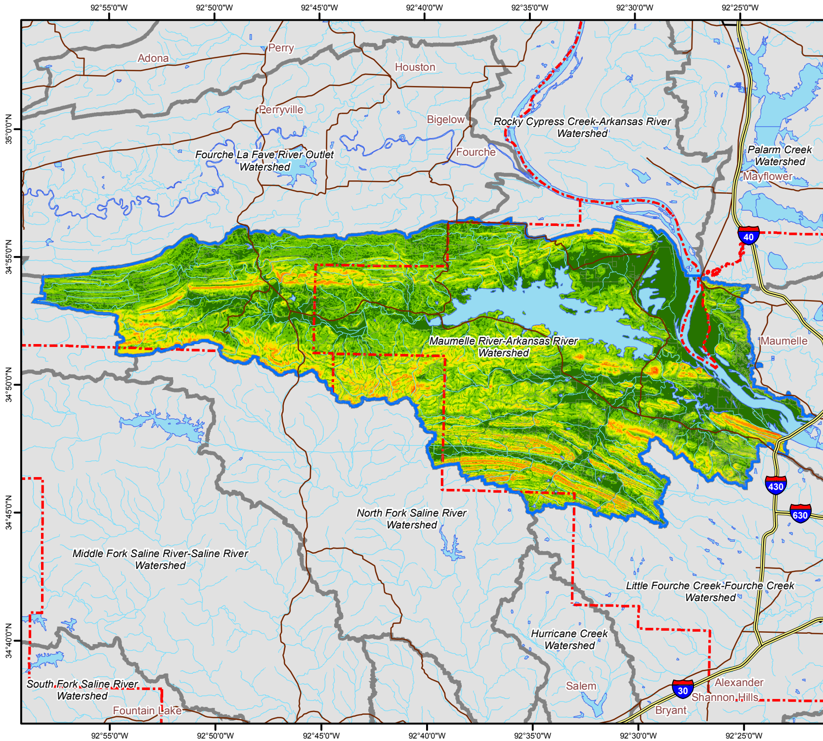
Maumelle River-Arkansas River Slope (Degrees)
