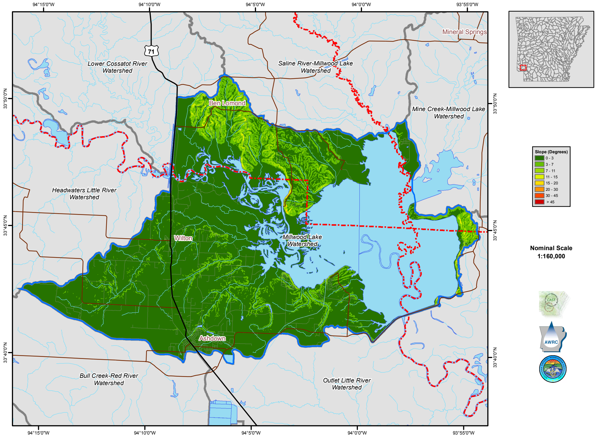
Millwood Lake Slope (Degrees)
